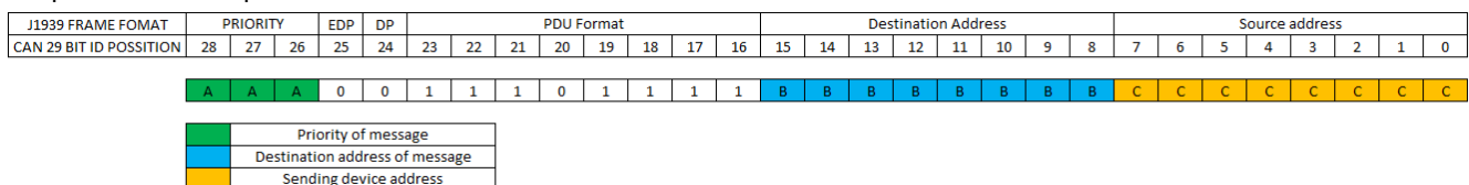
Figure 4 Proprietary A extend ID.
