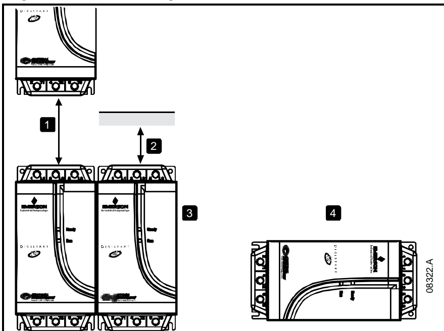
Figure 3-2 Distances de montage
