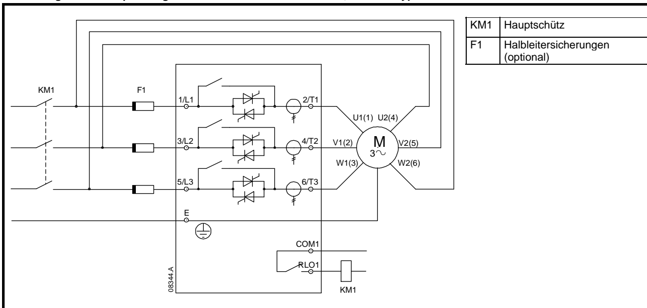
Abbildung 4-13 Hochspannungsanschlüsse - In-delta-Installation, interner Bypass
