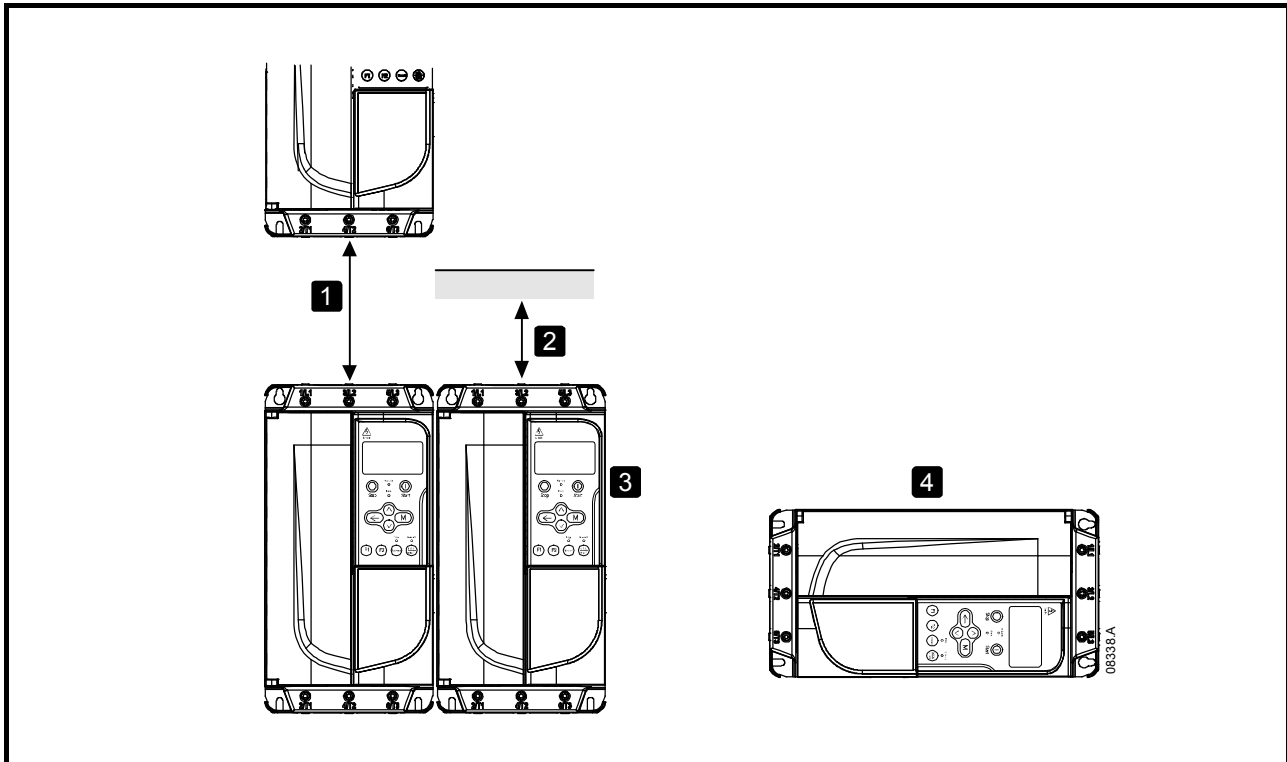
Figure 3-3 Distances de montage
