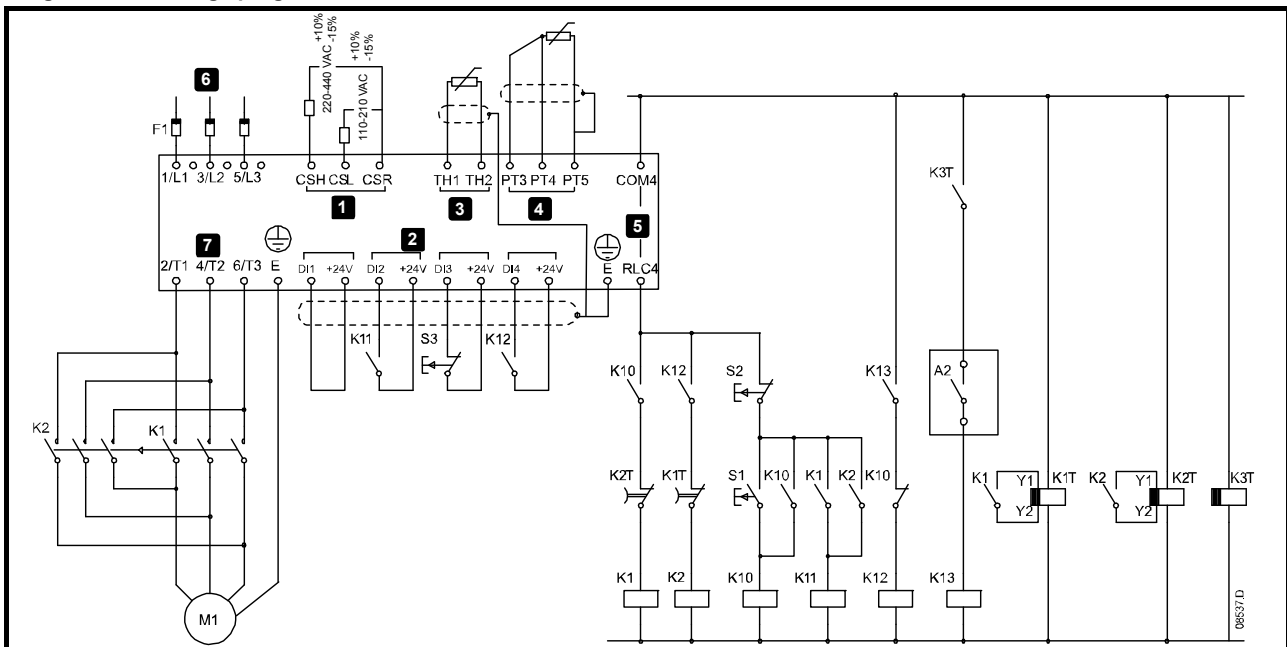
Figure 10-6 Freinage progressif
