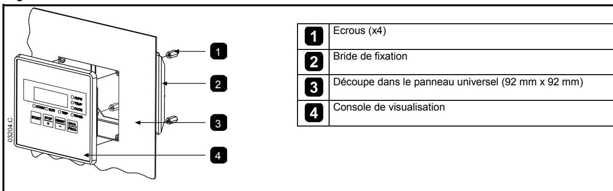
Figure 2-2 Installation
