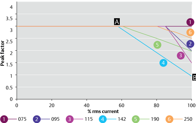
Standard peak torque factor
