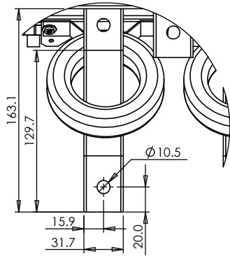
DETAIL C SCALE 1 : 3
